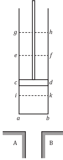
Figure 5: Sadi Carnot's diagram (redrawn) for a reversible heat engine to produce a net work output [11].
