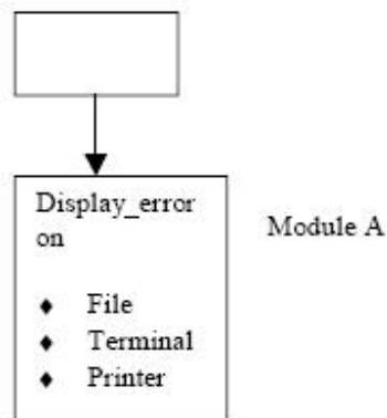
Fig. 6.7 Logical Cohesion
