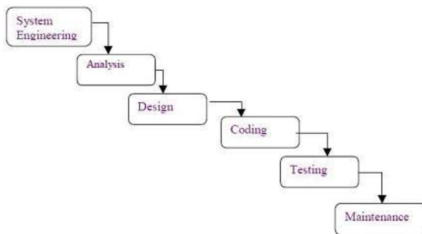
Fig2.2: Waterfall Model
