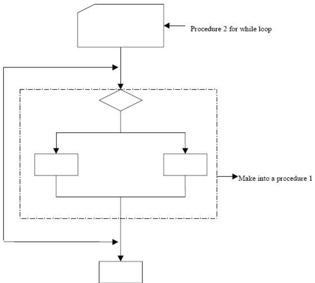
Fig. 6.6 Procedural cohesion
