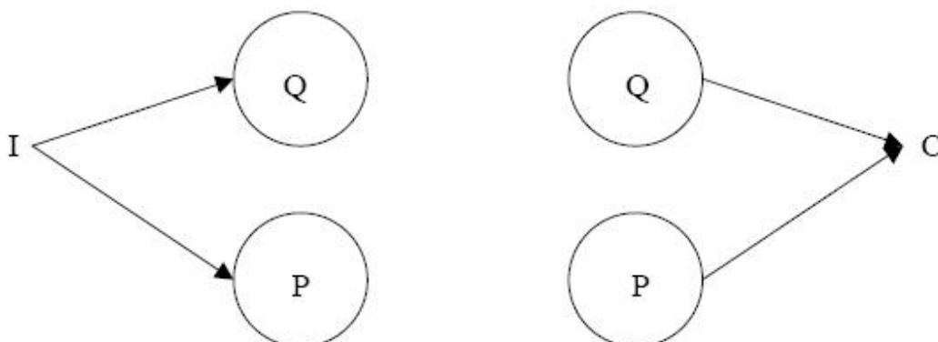
Fig. 6.5 Communicational cohesion
